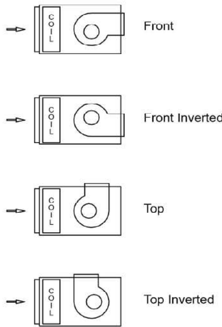
Horizontal arrangement unit
