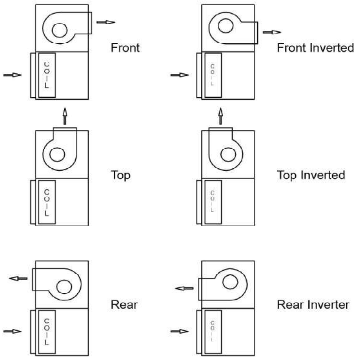
Vertical arrangement unit
